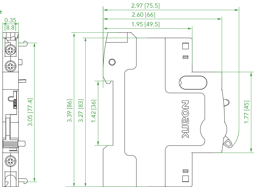
AL31/AX31 Alarm Switch/Auxiliary Contact Unit: in [mm]
