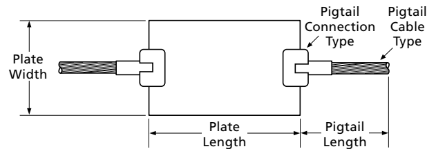
Through Pigtail
