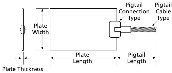
Terminated Pigtails
